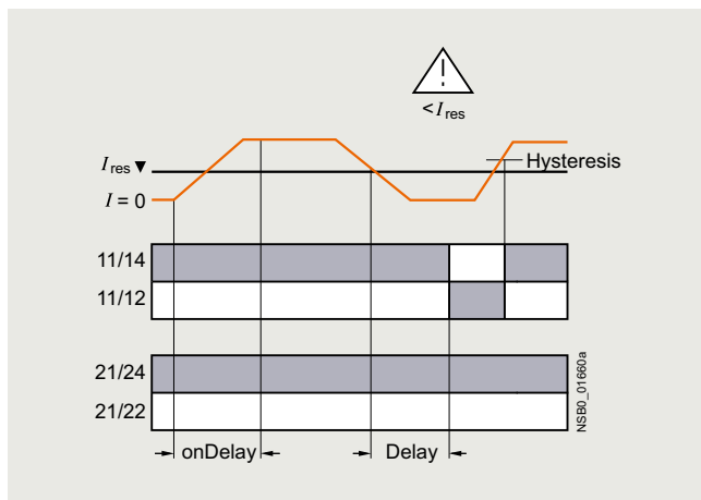
Undershooting of active current
