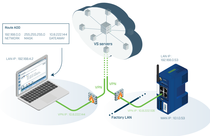
Figure 4-3: the eCatcher software automatically adds a route to the LAN IP address of the destination Ewon gateway.
