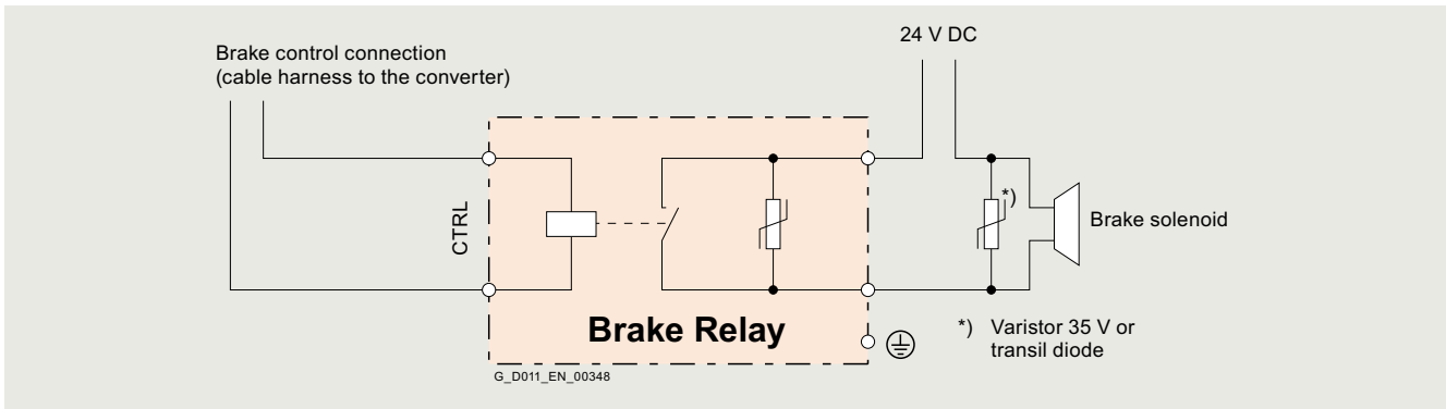
Connection example of 24 V DC Brake Relay
